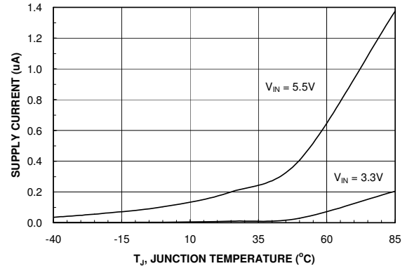
Figure 6. Reverse Current vs. Temperature
